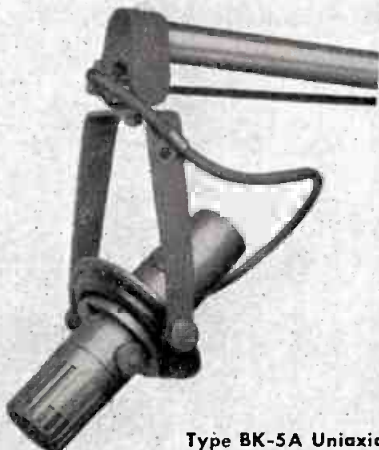
Type BK-5A Uniaxial Microphone with Boom Mount. Specially engineered for the television industry to reduce camera noise and interference. Newly designed boom mount combines superior mechanical isolation with rugged durability. Also available with wind screen for outdoor use.
